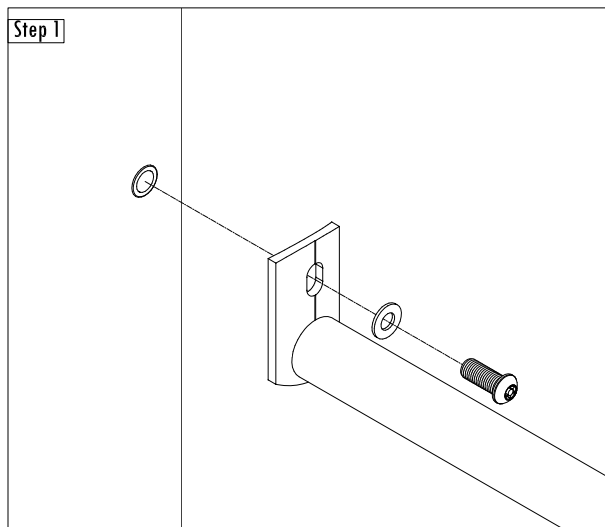
1" Button Cap, Flat Washer (x5)
