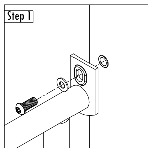
1" Button Cap Torx, Flat Washer (x1)
