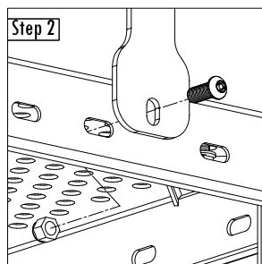
1" Button Cap Torx, Flat Washer, Lock Nut (x4)
