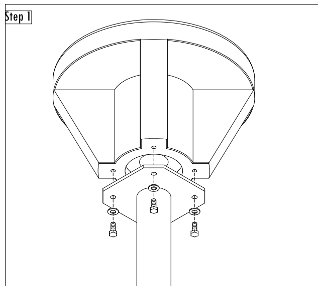
1" Machine Bolt, Flat Washer (x4)
