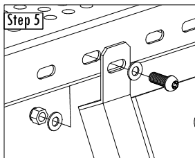
1" Button Cap Torx, Flat Washer, Lock Nut (x2)
