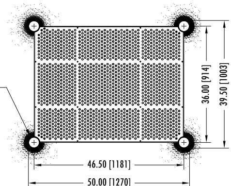
Playsteel FIT Rectangle Deck 3.5" Round Post
